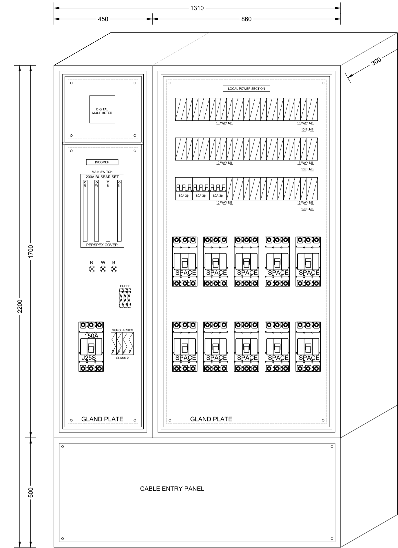
ESSENTIAL DISTRIBUTION BOARD
