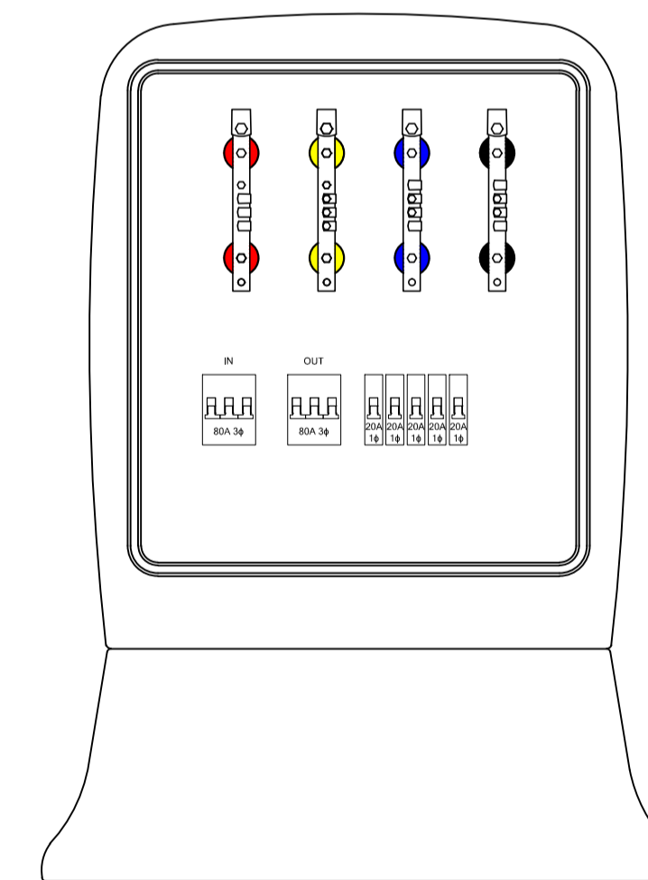
TYPICAL 9-WAY KIOSK ELECTRICAL SECTION
