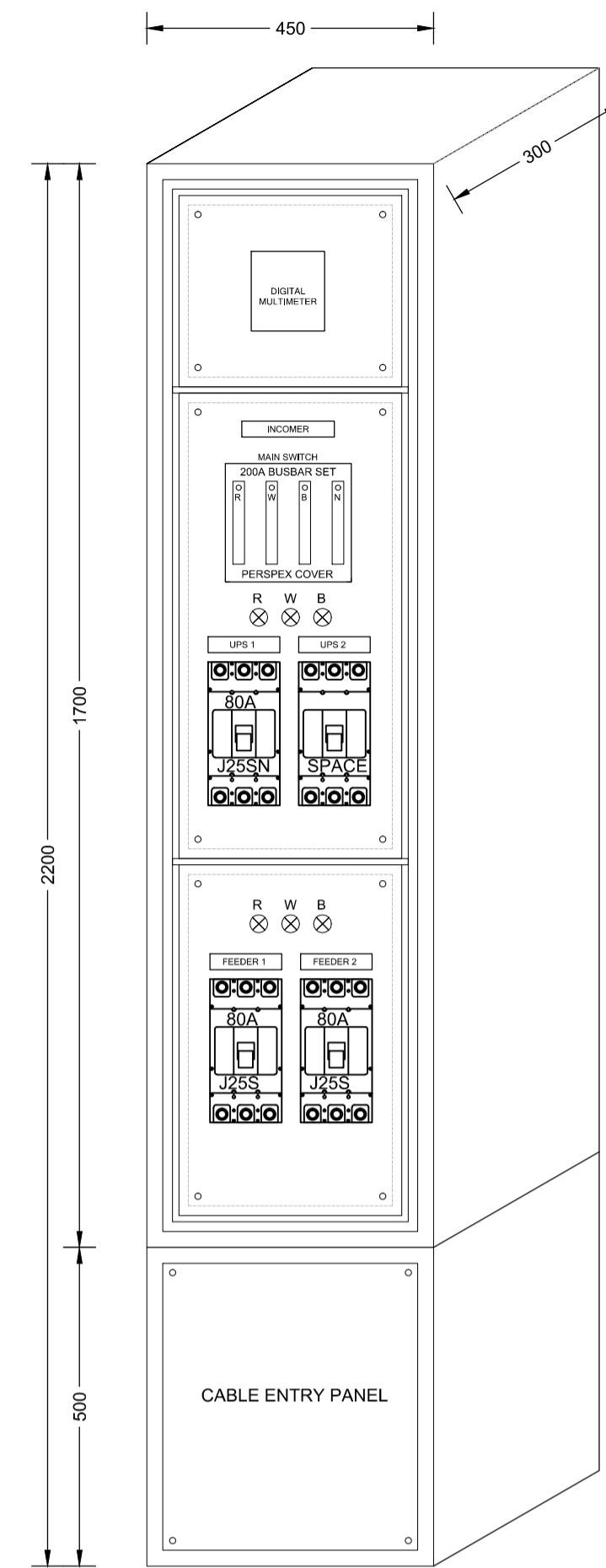
UPS DISTRIBUTION BOARD
